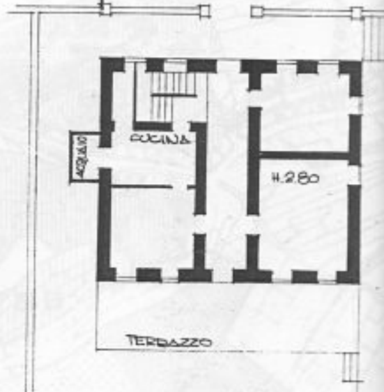
PIANO SEMINTERRATO
